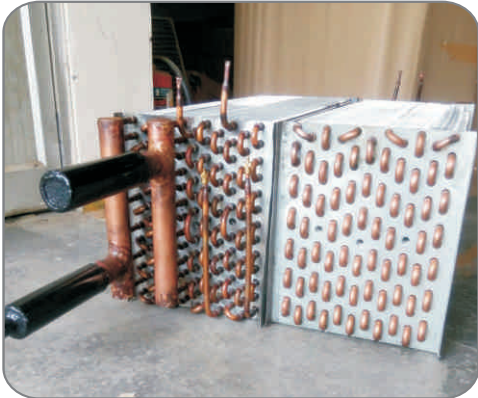
COOLING COIL CHILLED WATER AND DX COMBIND
